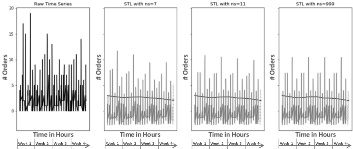
Fig. 4. STL decompositions for a medium-demand pixel with hourly time steps and periodicity k = 84 .
