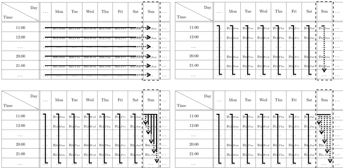
Fig. 5. Classification of the models by input type and training moment.
